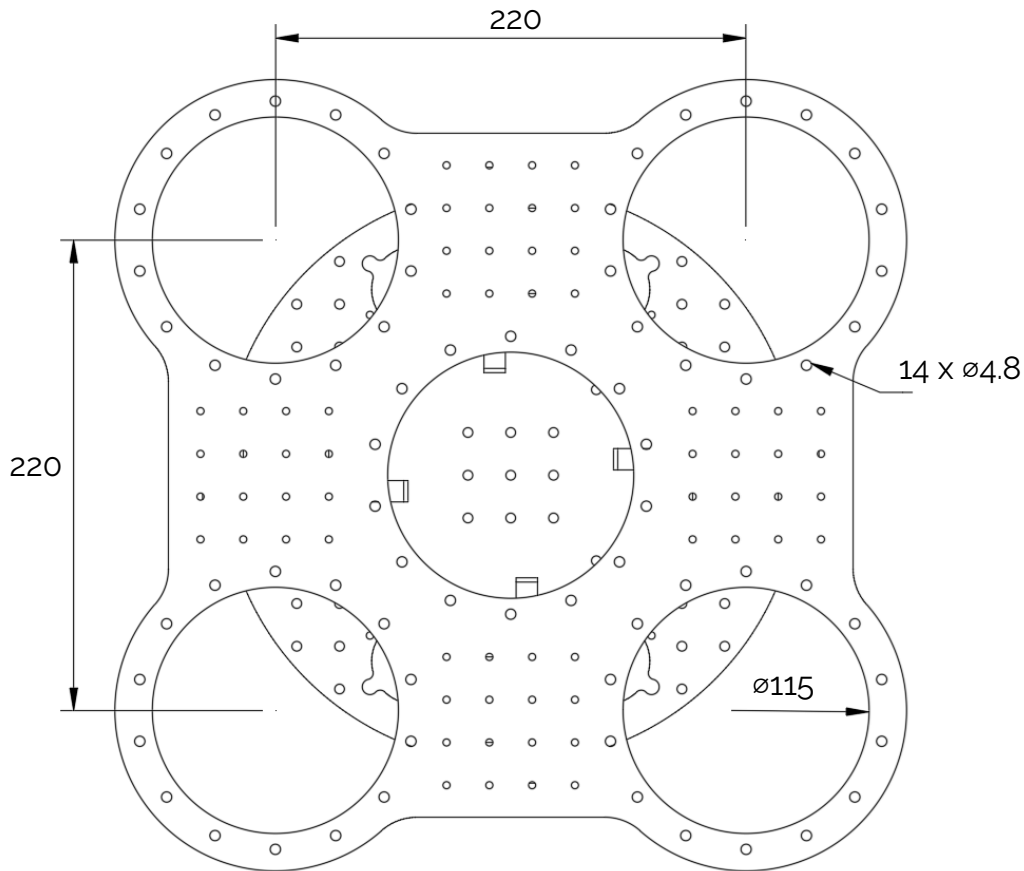
Drawing Coldstage – Bottom View [mm]
