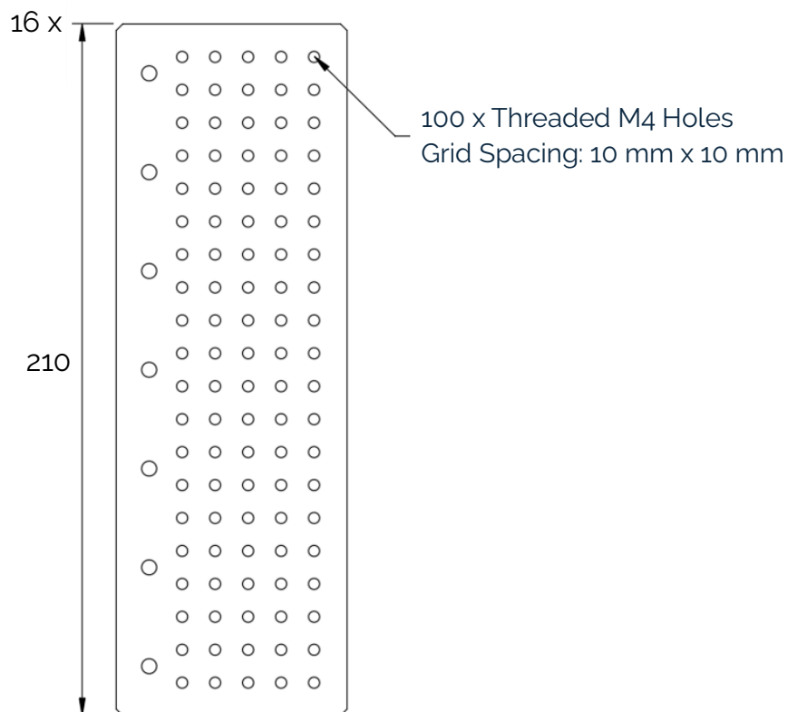
Drawing Breadboard – Side View [mm]
